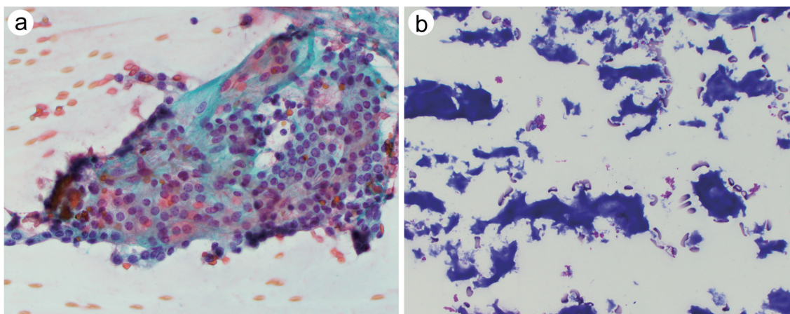
Fig. 3. Benign (consistent with follicular nodular disease). (a) Follicular groups arrange in flat sheets. Follicular cells are small (similar size as adjacent red blood cells) and evenly spaced with no nuclear enlargement, crowding, or overlapping. The cells have round to oval nuclei, evenly granular chromatin, and a scant or moderate amount of cytoplasm (smear, Pap stain). (b) Adjacent colloid is present (smear, Diff-Quik stain).
