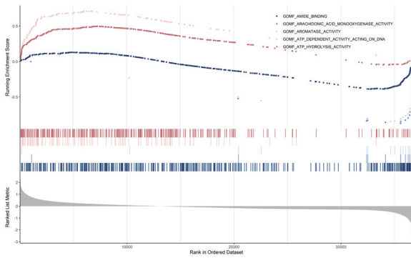
Supplement Figure 4. GO enrichment analysis in low-risk and high-risk group.
