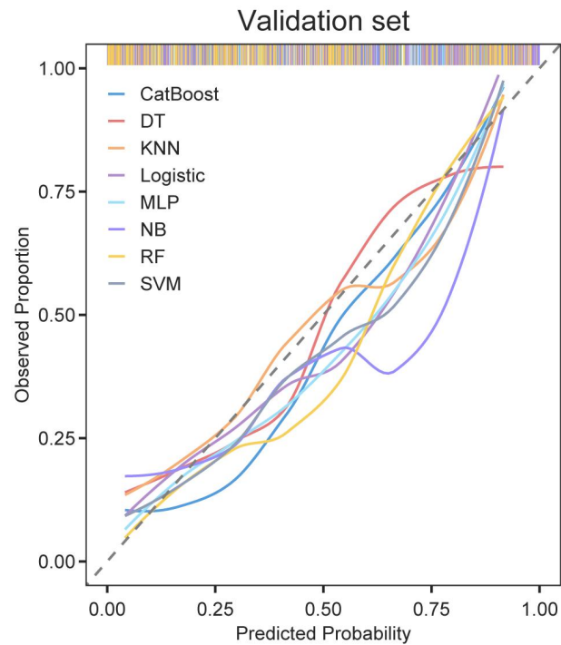
Supplementary Figure S8. Calibration curve of the six-metabolite model trained by eight ML models in the validation set. Note: ACLF, acute-on-chronic liver failure, CatBoost, Categorical boosting; DT, decision tree; KNN, K-nearest neighbor; Logistic, logistic regression; ML, machine learning; MLP, multilayer perceptron; NB, naive bayes; RF, random forest; SVM, support vector machine.
